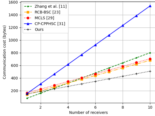
Fig. 6. Communication cost comparison of signcryption
