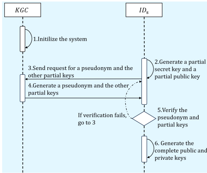
Fig. 2. Workflow of Setup, Partial Key Generation, and Complete Key Generation
