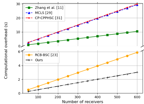
Fig. 4. Computational overhead comparison of signcrypton
