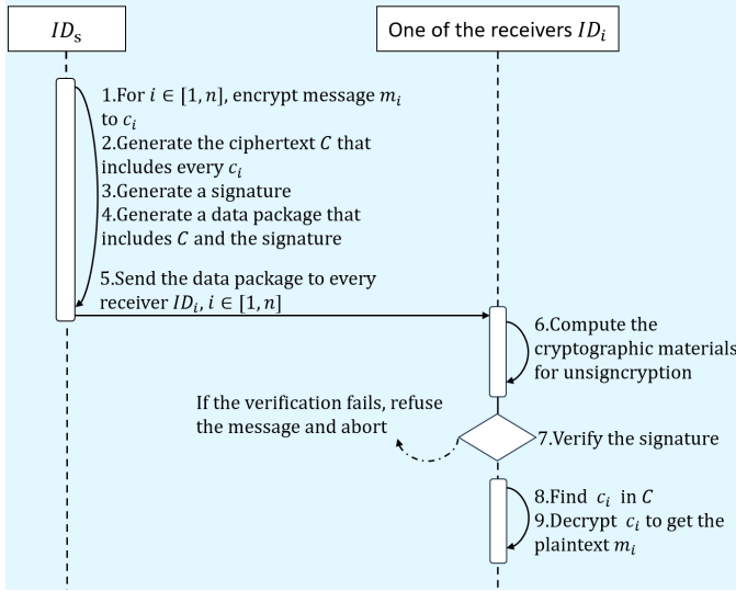
Fig. 3. Workflow of Multi-receiver Signcryption and Multi-receiver Unsigncryption
