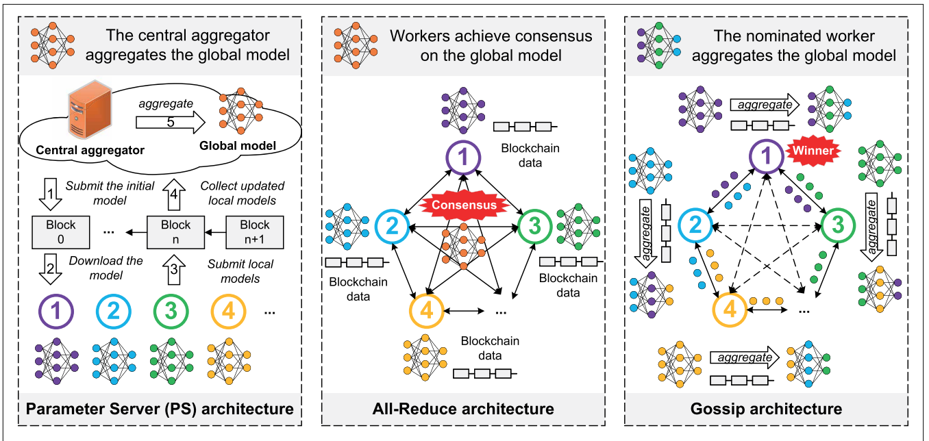
FIGURE 2. Three basic model aggregation architectures of BFL systems.
