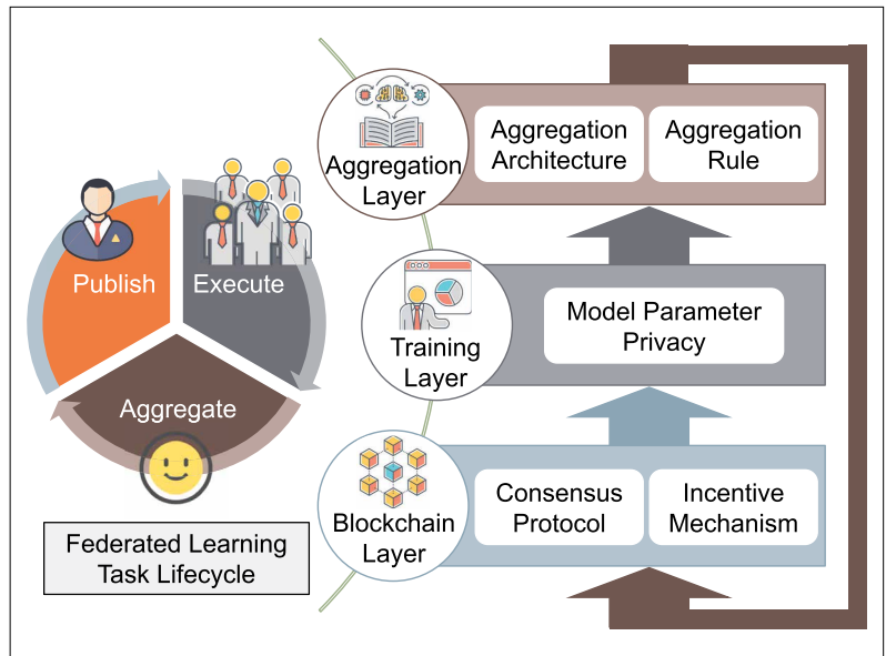
FIGURE 1. Taxonomy of BFL systems corresponding to the FL task lifecycle.
